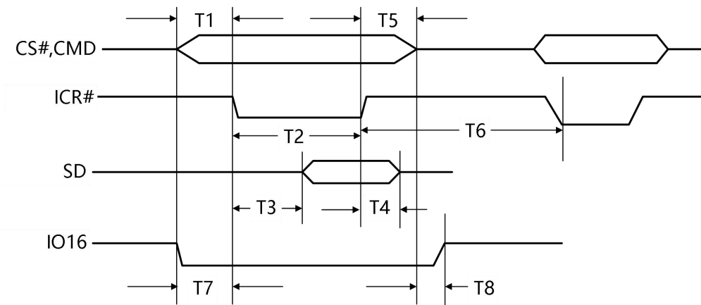
Figure 4. Processor Read Timing
