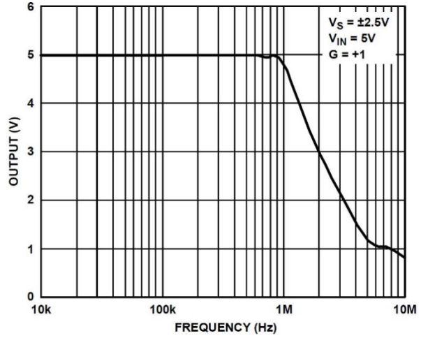
Figure 24. Maximum Output Swing vs. Frequency
