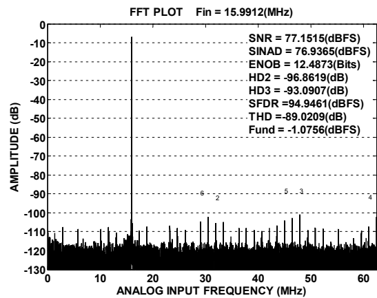
Figure14.Single-Tone 32K( f_{IN}=16\text{MHz} , f_s=125\text{MSPS} )
