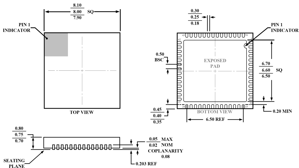
Figure 63.56 Pin lead packaging (plastic packaging)
