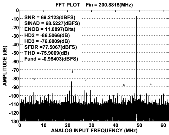
Figure17.Single-Tone 32K( f_{IN}=201\text{MHz} , f_s=125\text{MSPS} )
