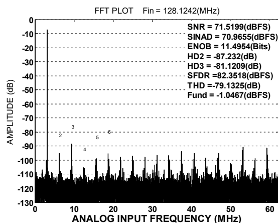
Figure 8. Single-Tone 32k ( f_{IN} = 128\text{ MHz} , f_s = 125\text{ MSPS} )
