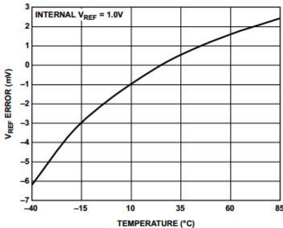
Figure 38. V REF Error vs. Temperature, Typical V REF = 1.0 V Drift Figure 39. V REF Error vs. Temperature, Typical V REF = 1.4 V Drift
