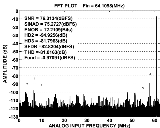
Figure 7. Single-Tone 32k ( f_{IN} = 64\text{ MHz} , f_s = 125\text{ MSPS} )
