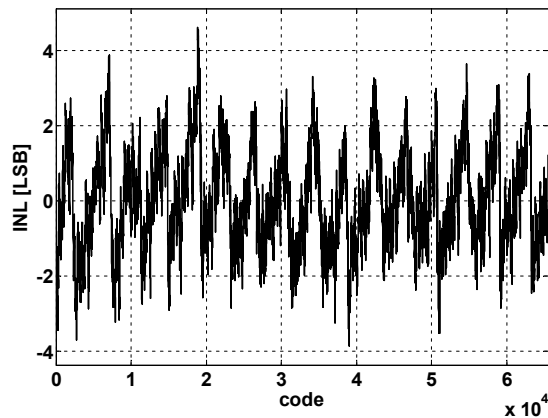
Figure20.Integral Nonlinearity (INL)( f_{IN}=10\text{MHz} , f_s=125\text{MSPS} )
