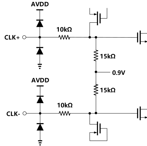
Figure 22. Equivalent CLOCK Input Circuit
