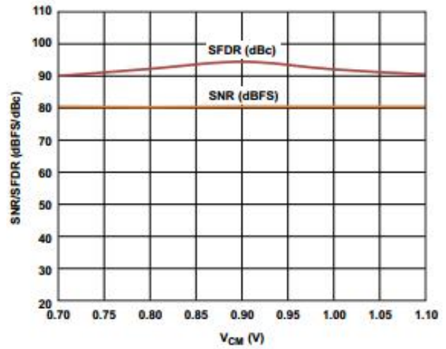
Figure 31. SNR/SFDR vs. Common-Mode Voltage (V CM ), (f IN =9.7MHz, f SAMPLE =125MSPS, V REF =1.4V)
