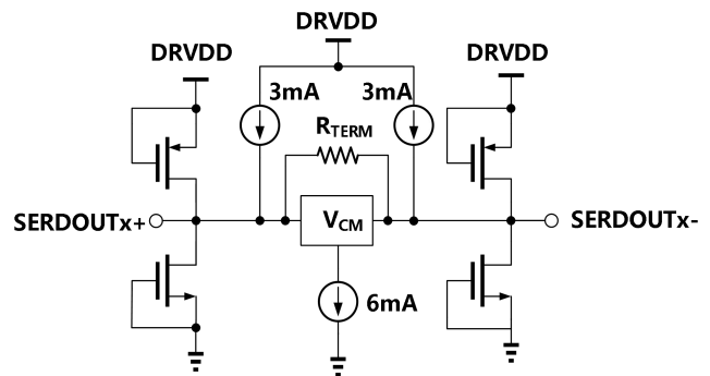
Figure 24. Equivalent SERDOUT± Circuit
