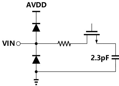
Figure 21. Equivalent Analog Input Circuit
