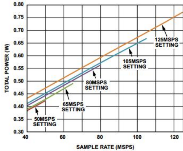
Figure 46. Total Power vs. f_{SAMPLE}
