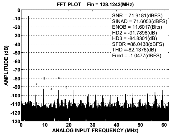
Figure16.Single-Tone 32K( f_{IN}=128\text{MHz} , f_s=125\text{MSPS} )
