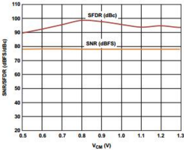
Figure 30. SNR/SFDR vs. Common-Mode Voltage (V CM ), (f IN =9.7MHz, f SAMPLE =125MSPS, V REF =1.0V)
