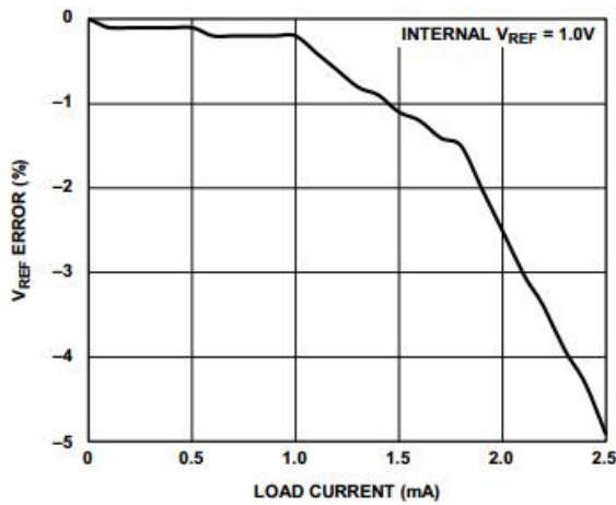
Figure 36. V REF Error (Internal V REF = 1.0 V) vs. Load Current Figure 37. V REF Error (Internal V REF = 1.4 V) vs. Load Current
