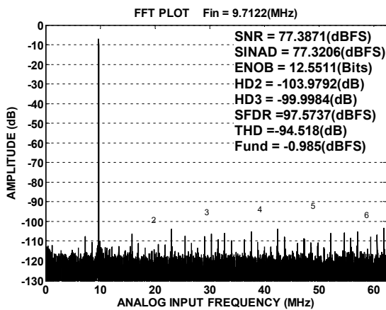
Figure13.Single-Tone 32K( f_{IN}=9.7\text{MHz} , f_s=125\text{MSPS} )
