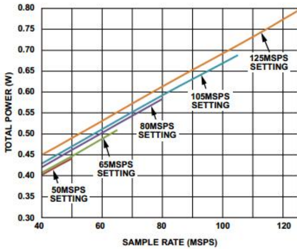
Figure 45. Total Power vs. f_{SAMPLE}
