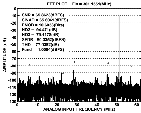
Figure18.Single-Tone 32K( f_{IN}=301\text{MHz} , f_s=125\text{MSPS} )
