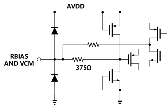
Figure 26. Equivalent RBIAS, VCM Circuit
