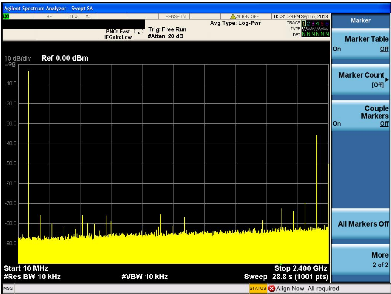
Figure 3. Single-Tone Spectrum at f_{OUT}=91\text{MHz} , f_{DAC}=2.4\text{GSPS}
