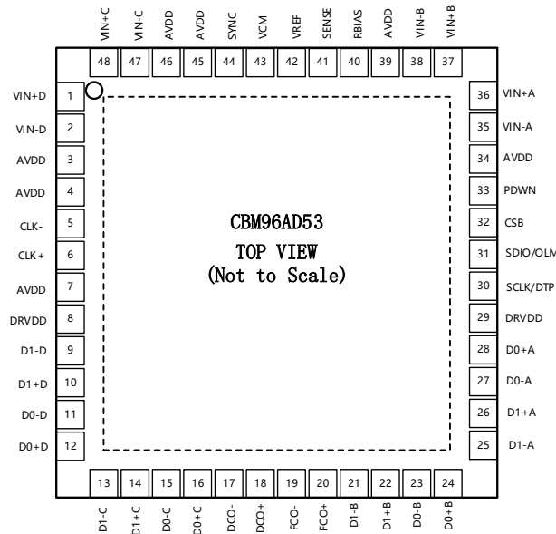
QFN-48 Pin Configuration, Top View
