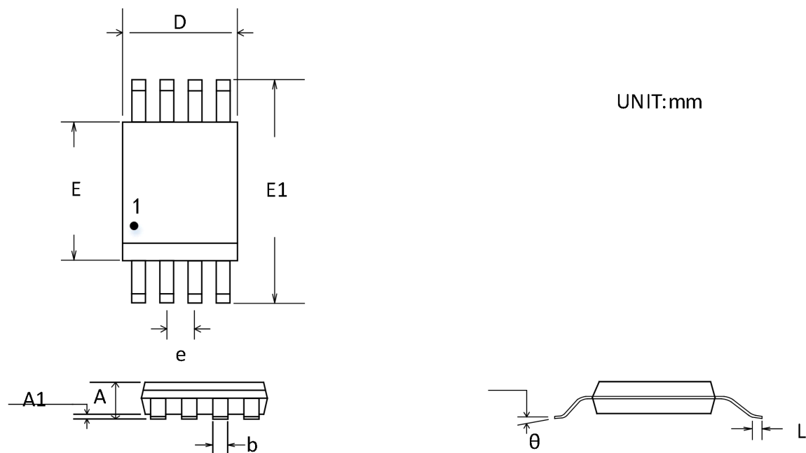
Figure 29. TSSOP-8 Outline Package
