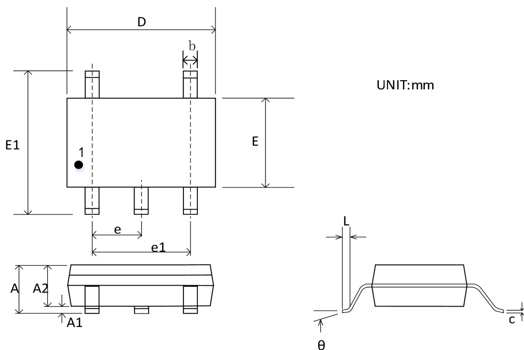
Figure 26. SOT23-5 Outline Package
