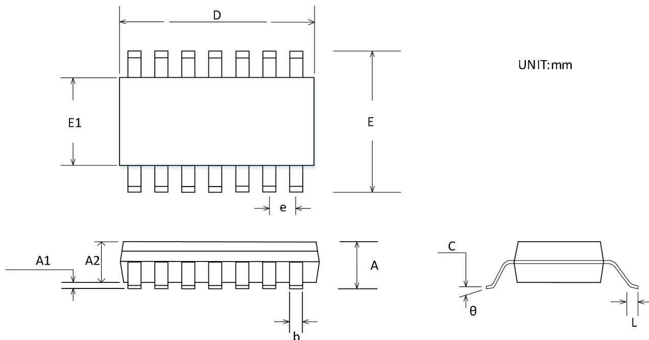
Figure 31. SOP-14 Outline Package
