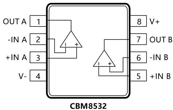
Figure 3. 8-Lead SOP, 8-Lead TSSOP-8 and 8-Lead MSOP (R, RU, and RM Suffixes)
