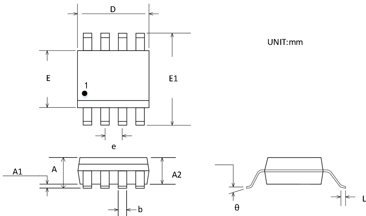
Figure 27. SOP-8 Outline Package
