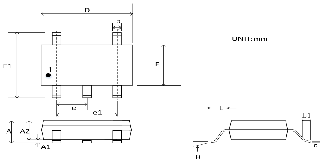
Figure 25. SC70-5 Outline Package
