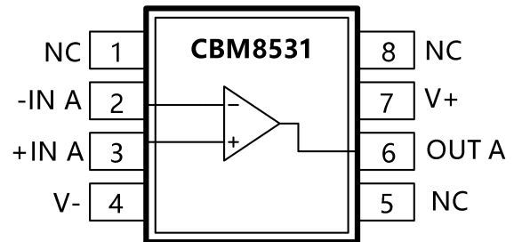
Figure 2. 8-Lead SOP (R Suffix)
