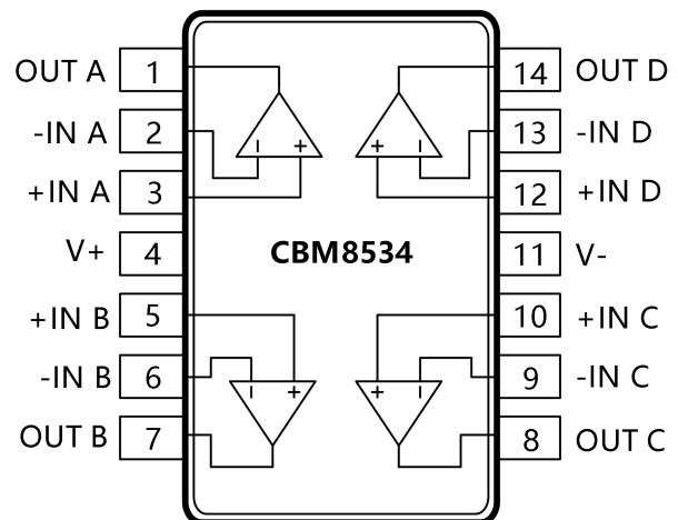
Figure 4. 14-Lead SOP and 14-Lead TSSOP (R and RU Suffixes)
