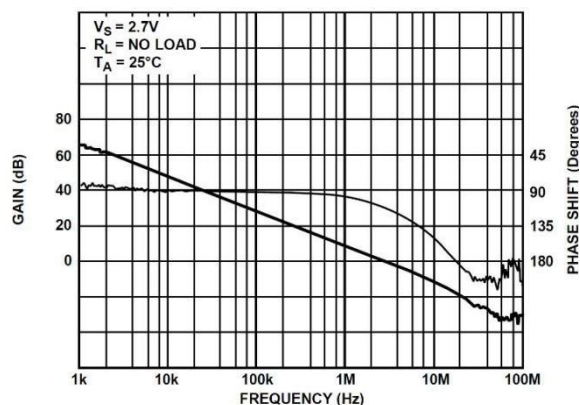
Figure 13. Open-Loop Gain and Phase Shift vs. Frequency
