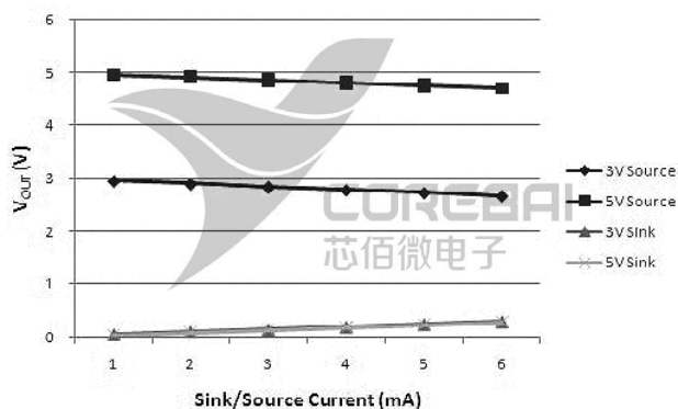
图 10. Vout Source and Sink Current Capability
