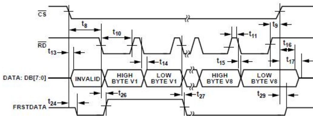
Figure 7. BYTE Mode Read Operation
