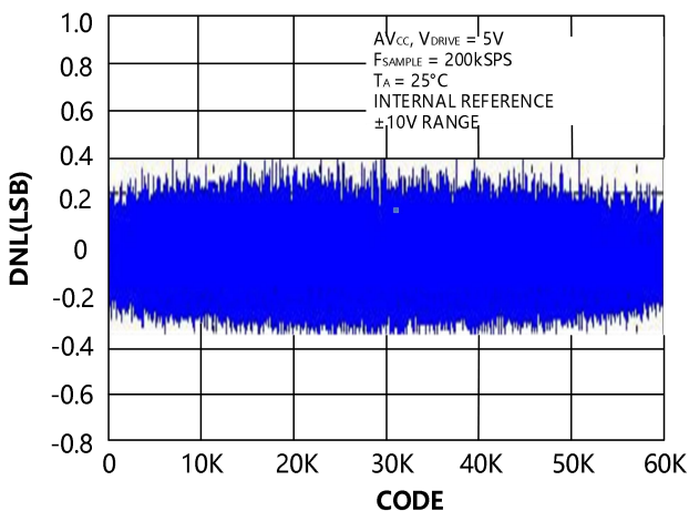
Figure 10. CBM76AD06 Typical DNL, \pm 10 V Range
