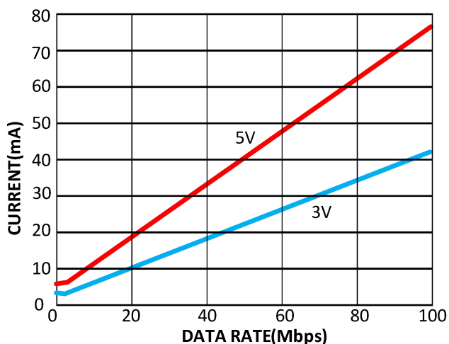
Figure 8. Typical CBMuD1400 V_{DD1} Supply Current vs. Data Rate for 5V and 3V Operation
