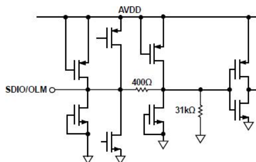
Figure 10. Equivalent SDIO/OLM Input Circuit
