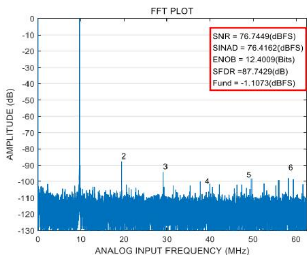
Figure 7. Single-tone 32K (fIN=10MHz, fS=125MSPS)
