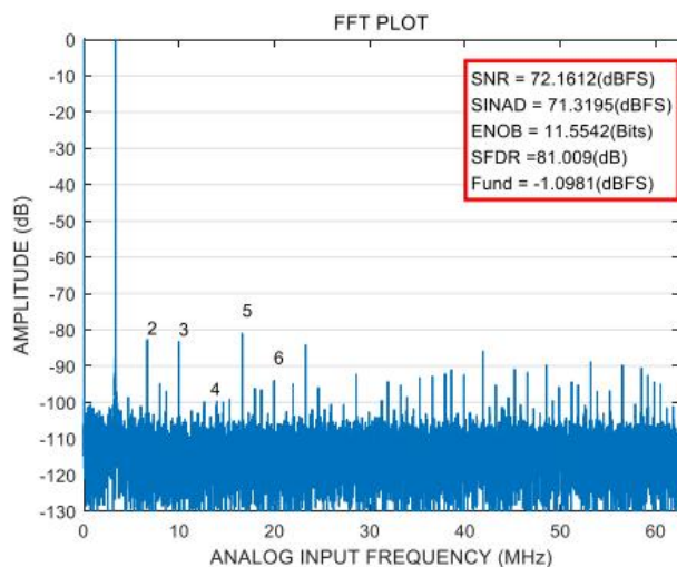
Figure 9. Single-tone 32K (fIN=128MHz, fS=125MSPS)
