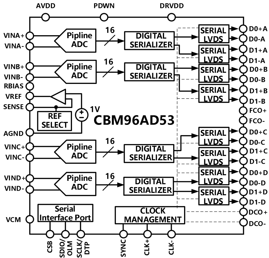
Figure 2. Block Diagram
