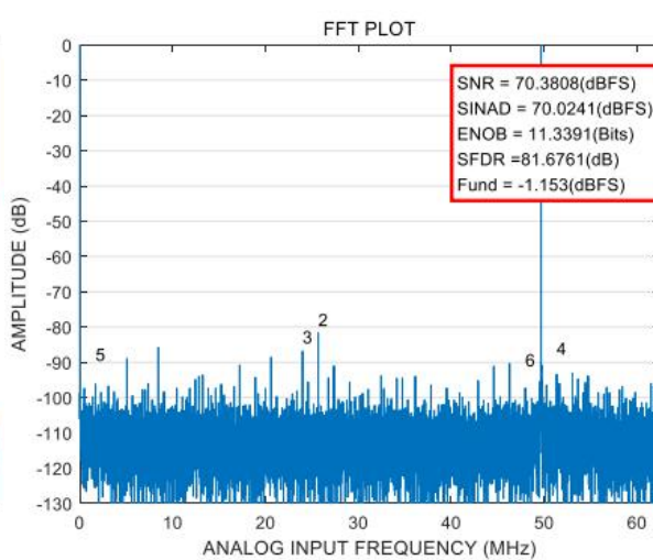
Figure 10. Single-tone 32K (fIN=200MHz, fS=125MSPS)
