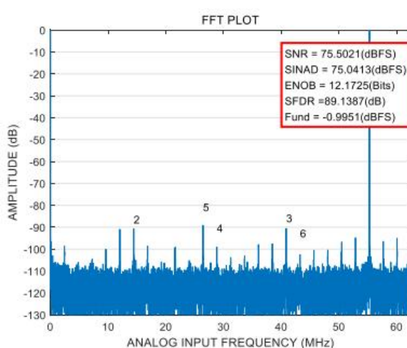
Figure 8. Single-tone 32K (fIN=70MHz, fS=125MSPS)
