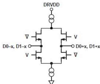
Figure 8. Equivalent Digital Output Circuit
