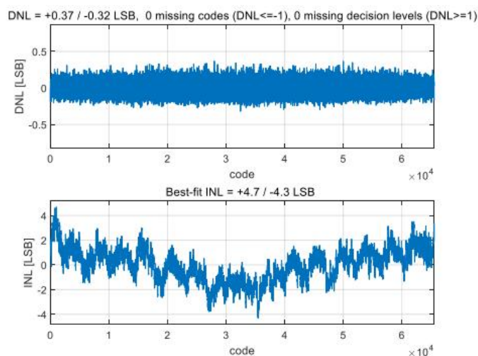
Figure 11.DNL/INL( f_{IN}=10\text{MHz} , f_S=125\text{MSPS} )
