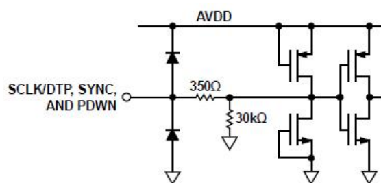
Figure 12. Equivalent SCLK/DTP, SYNC, and PDWN Input Circuit
