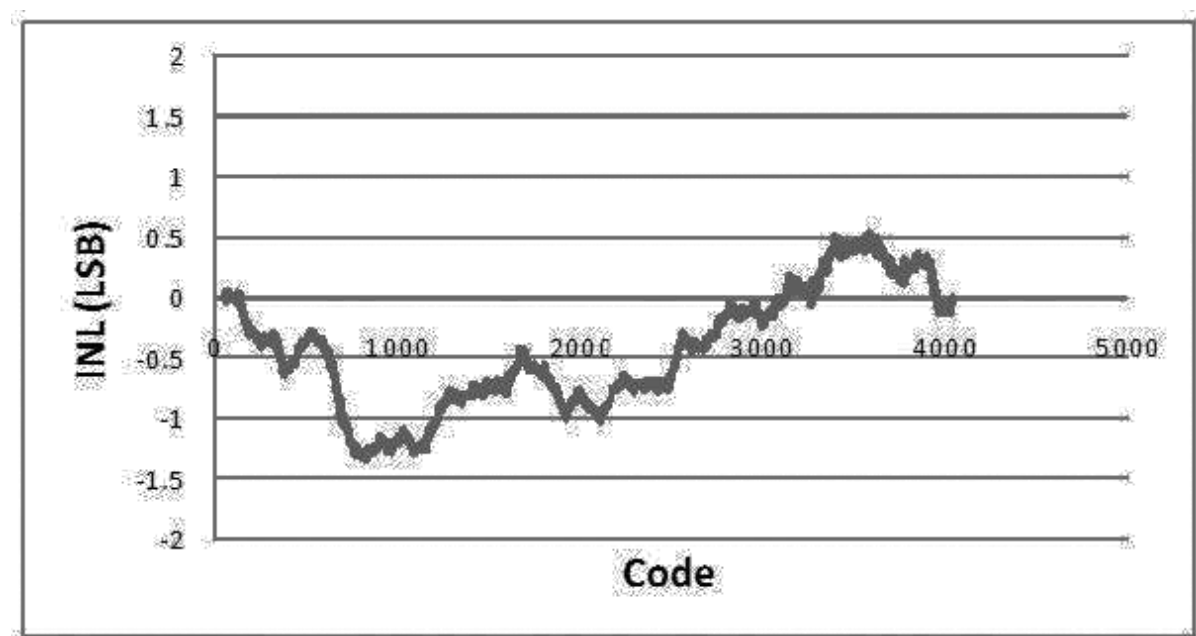
Figure 5. CBM128S085 typical INL
