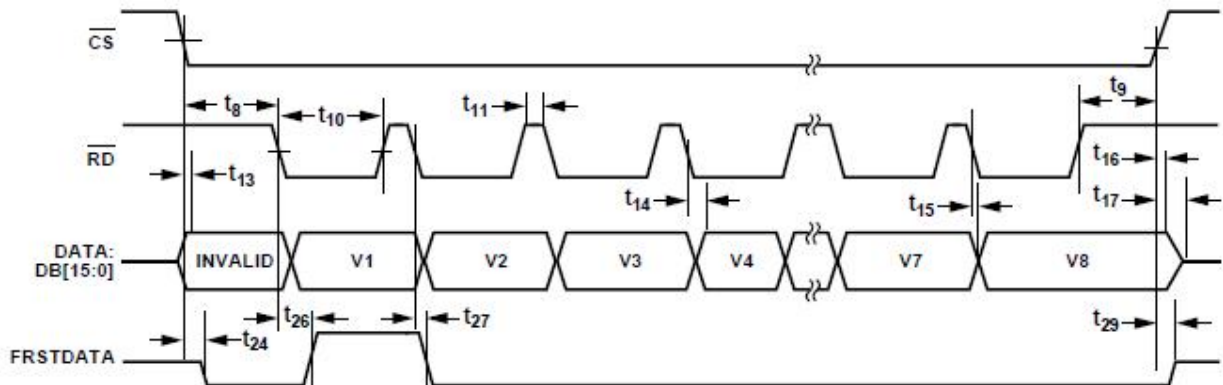
Figure 4. Parallel Mode, Separate \overline{CS} and \overline{RD} Pulses
