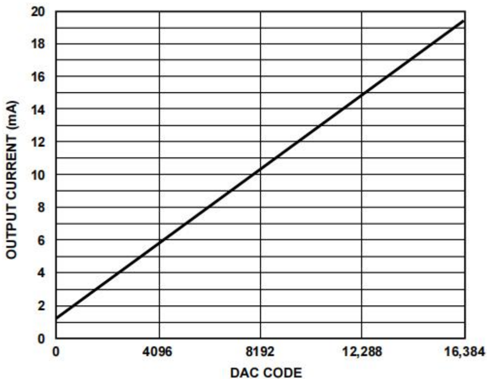
Figure 42. Gain Curve for \text{FSC}[9:0] = 512 , DAC Offset = 1.228 \text{ mA}
