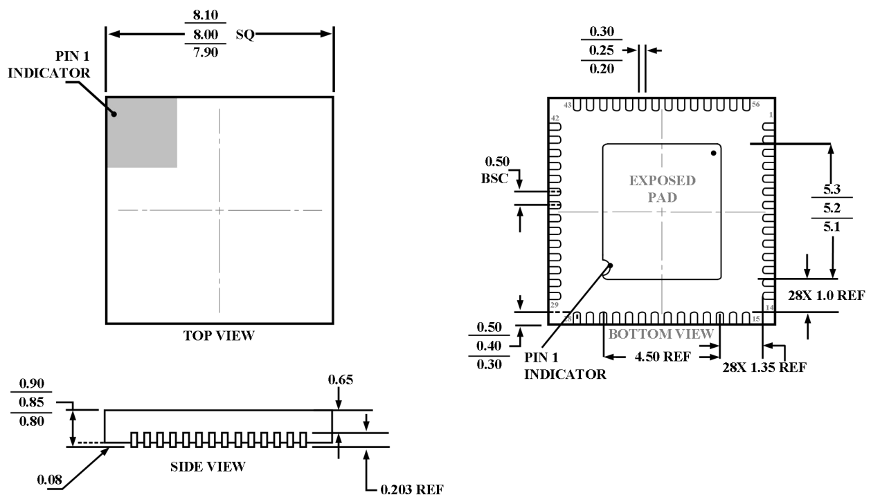
Figure 15. 56 Pin lead packaging (plastic packaging)
