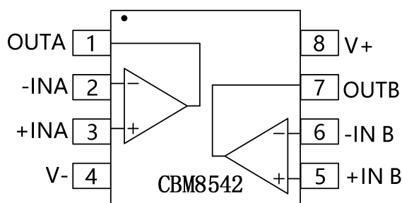
SOIC-8(SOP8)/MSOP-8/TSSOPP-8
