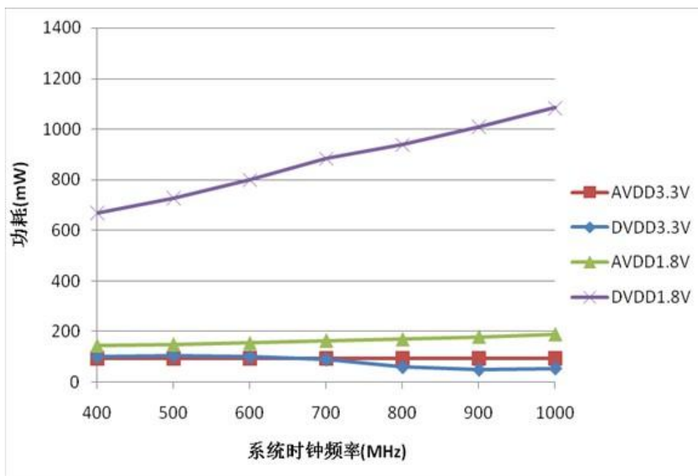
Figure 12. Power Dissipation vs. System Clock (PLL Enabled)
