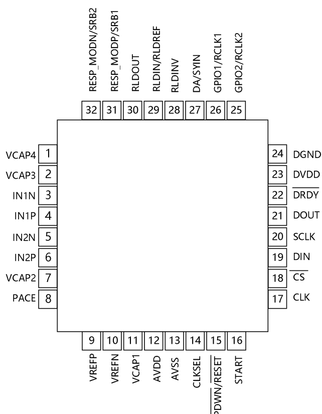
Figure 2. VQFN-32 Pin Configuration (Top View)
