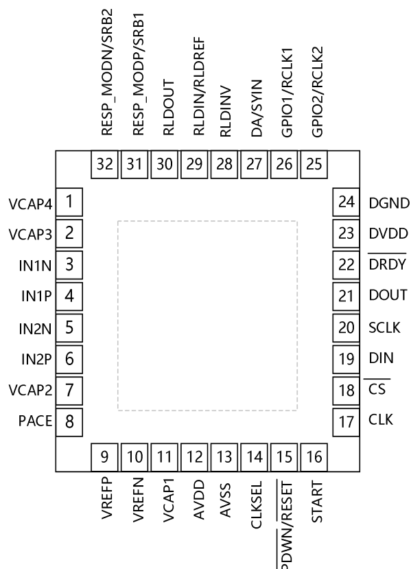
Figure 3. TQFP-32 Pin Configuration (Top View)
