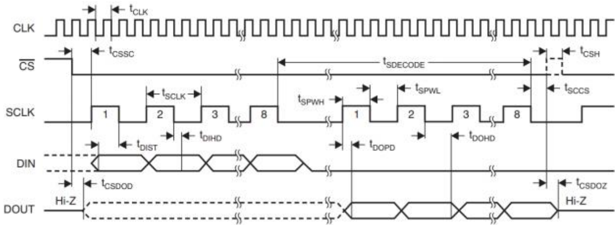
Serial Communication Timing Diagram
