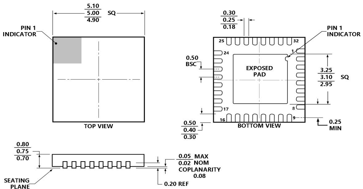
VQFN-32 Package Drawing
