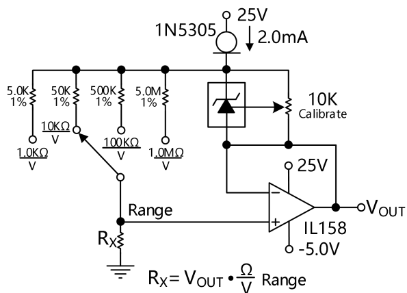
Figure 28. Linear Ohmmeter
