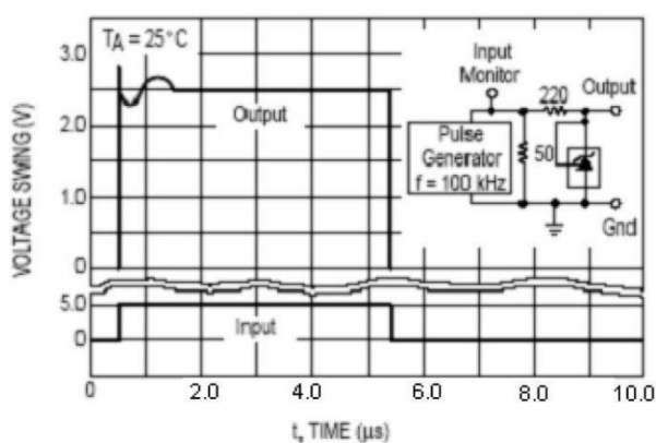
Figure 14. Pulse Response
