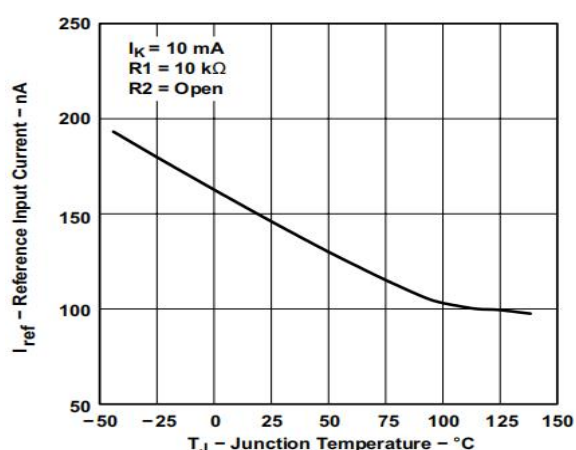
Figure 7. Reference Input Current versus Junction Temperature
