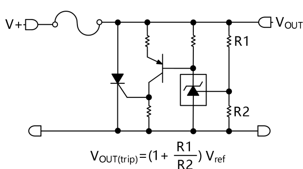
Figure 25. SRC Crowbar
