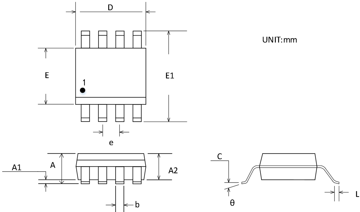
Figure 7 . 8-Lead Outline Package [MSOP-8]
