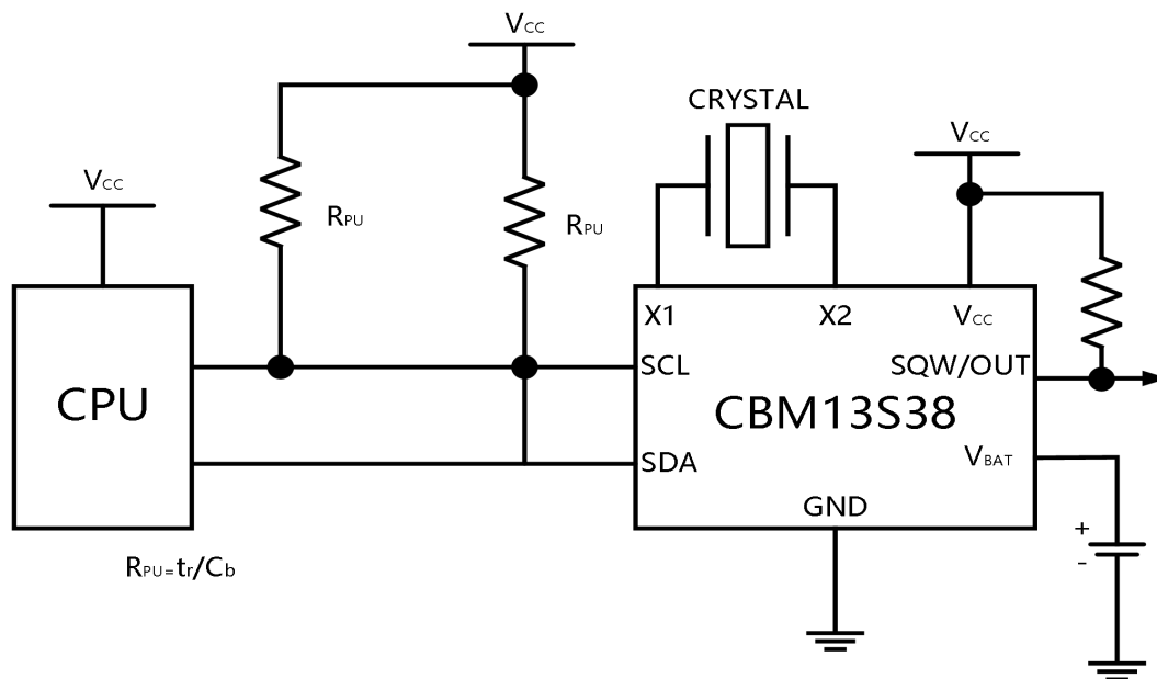
Figure 5. Typical Application Circuit Diagram
