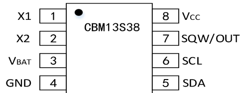
Figure 1. SOP8/MSOP8 Pin Configuration
