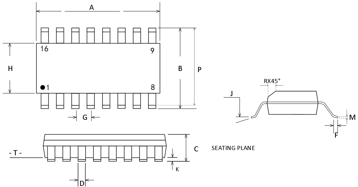
Figure 8 . 16-Lead Outline Package [SOP-16]
