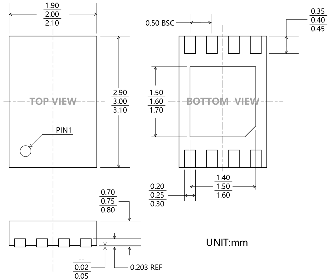
Figure 9 . 8-Lead DFN Package [DFN-8]
